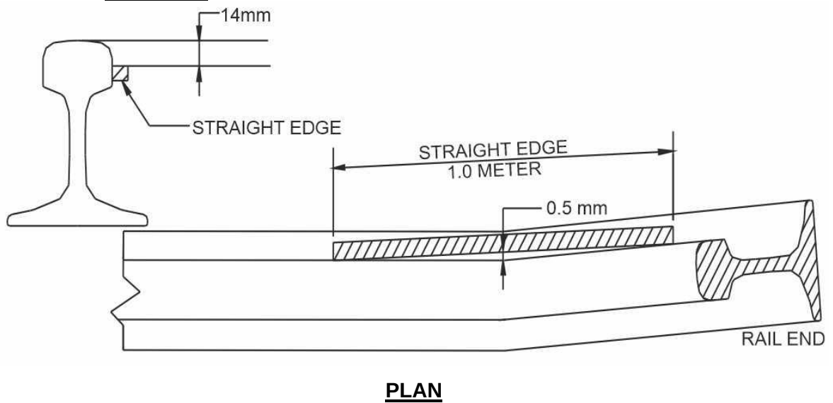
FIG: 3.1(c) Tolerance on the End Bends in the Horizontal Plane
