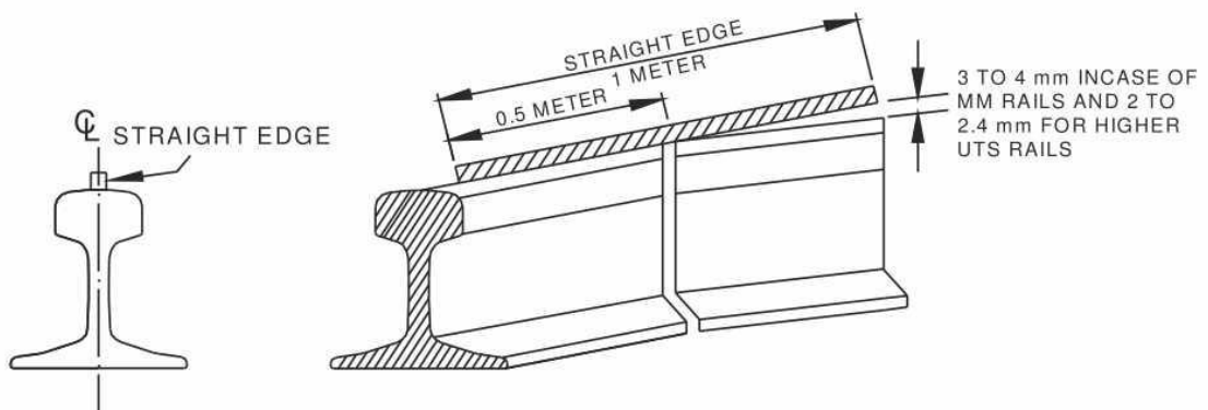
FIG: 3.2(c) Tolerance for Vertical Alignment at the Time of Welding
